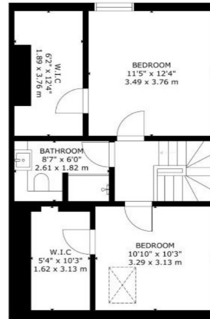
EXISTING SECOND FLOOR PLAN 1:100m
