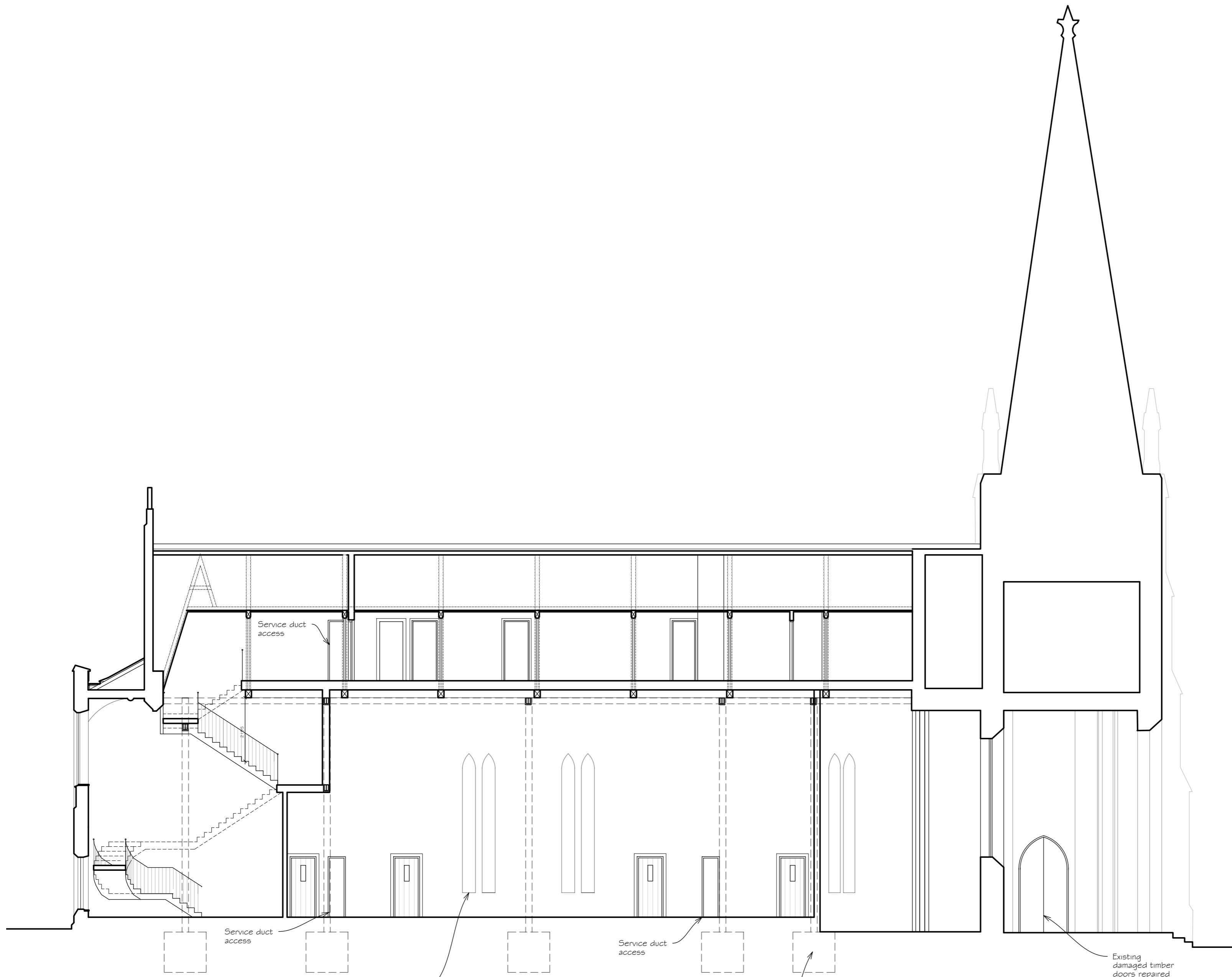
SECTION B For further information see also structural engineers drawings
