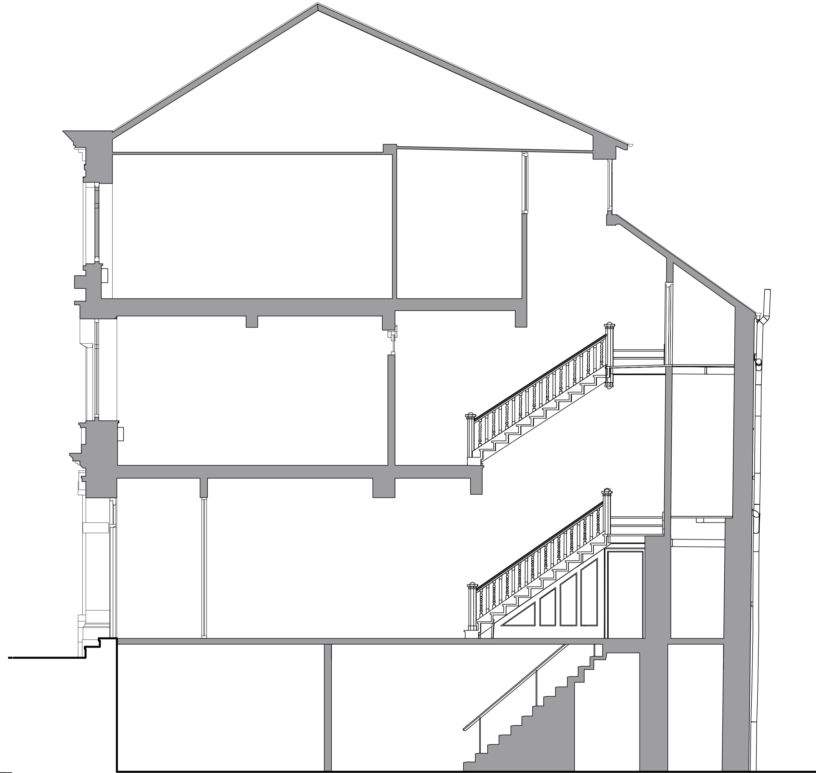
Section B - 1:50
