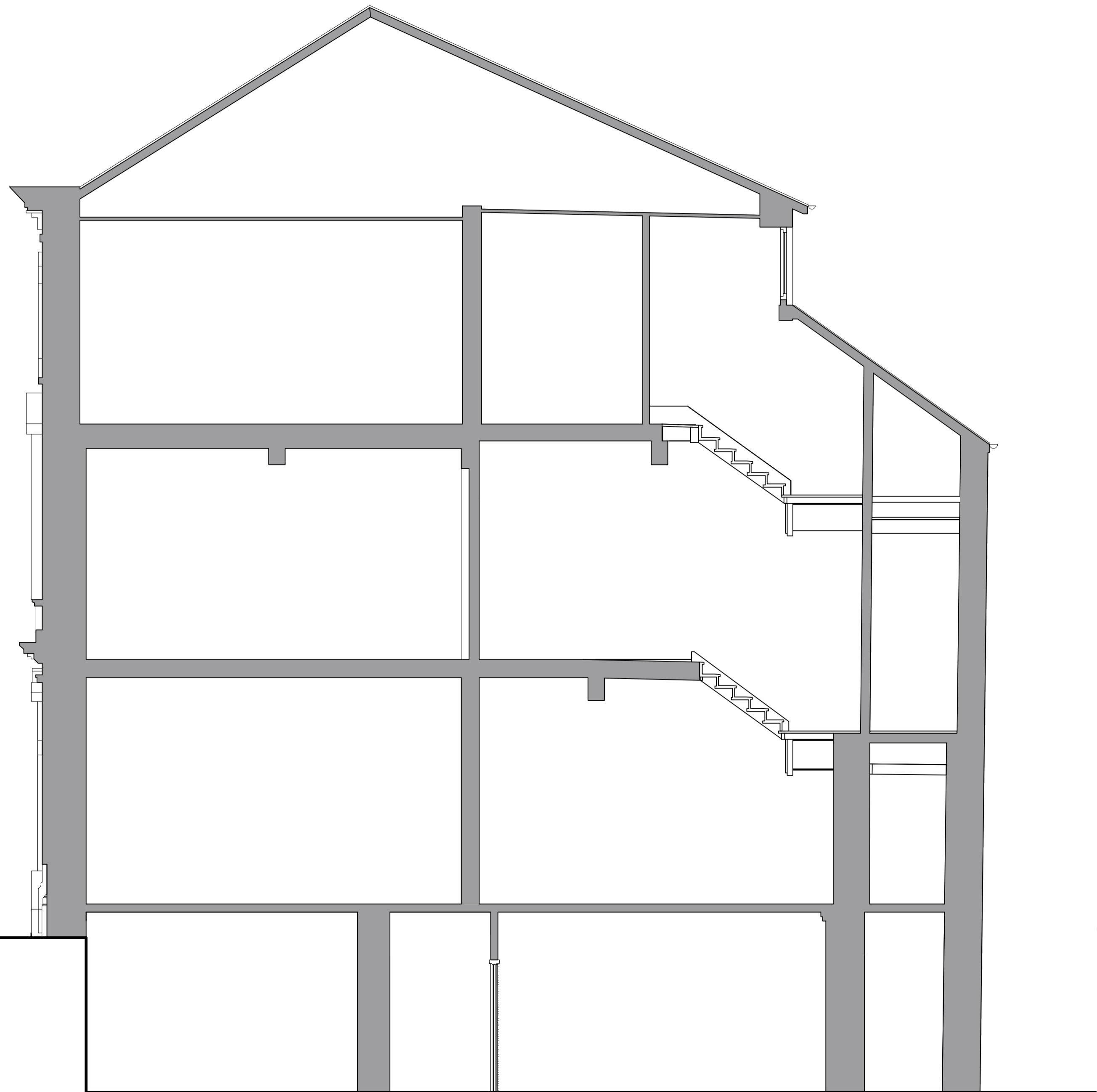
Section A - 1:50
