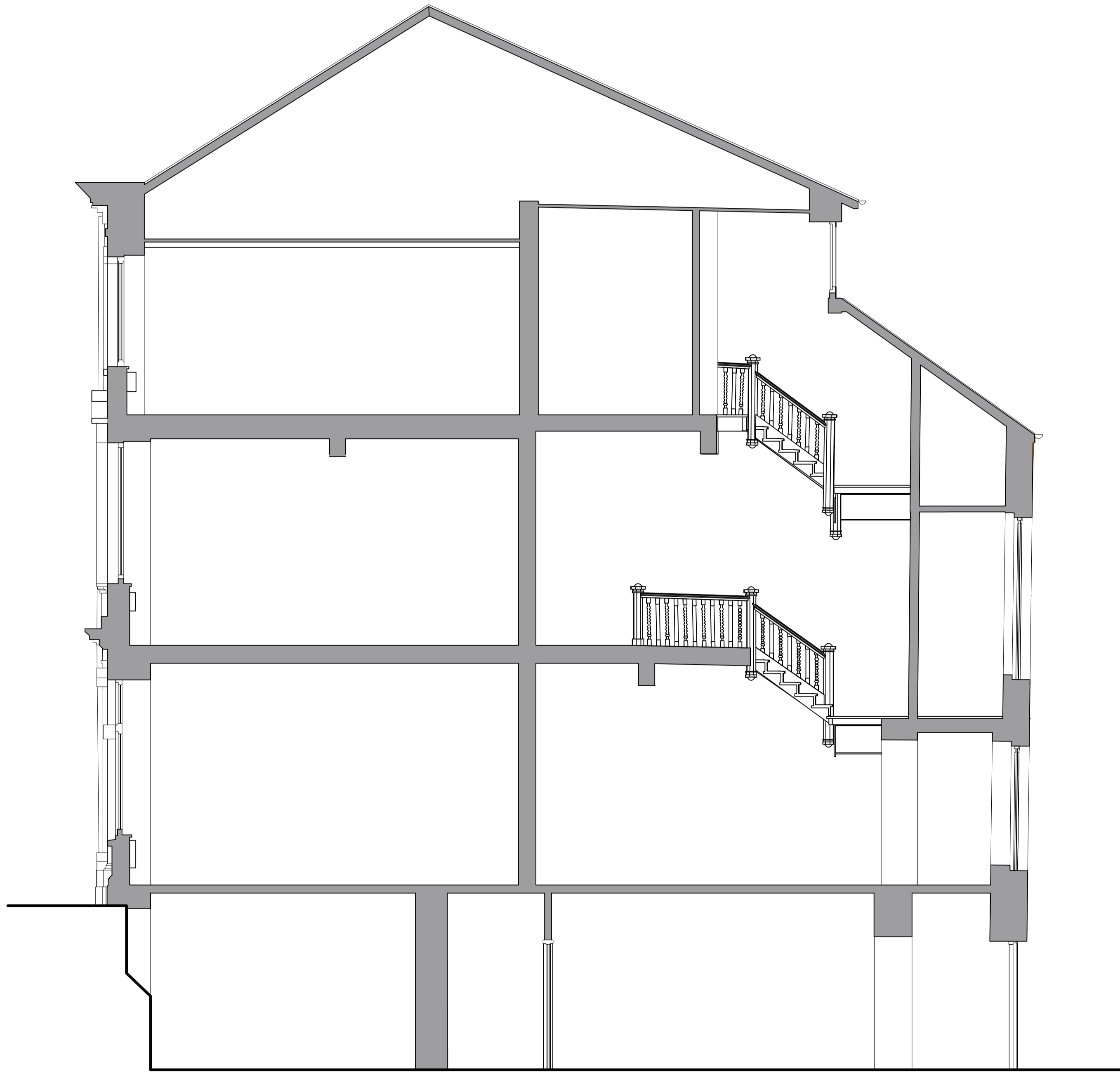
Section C - 1:50
