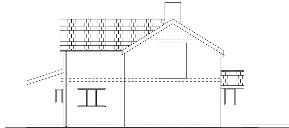
SIDE (WEST) ELEVATION
