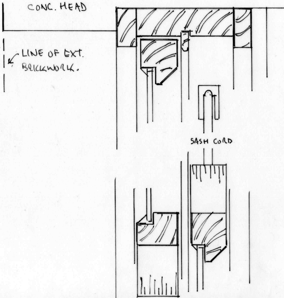
VERTICAL HEAD SECTION - EXG
