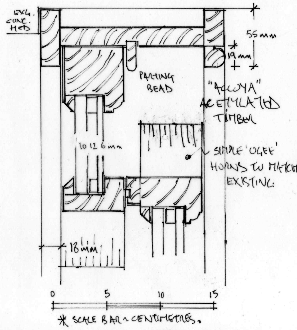
VERTICAL HEAD SECTION - PROPOSED
