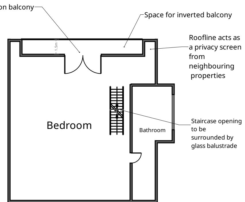
Proposed - First Floor Attic conversion
