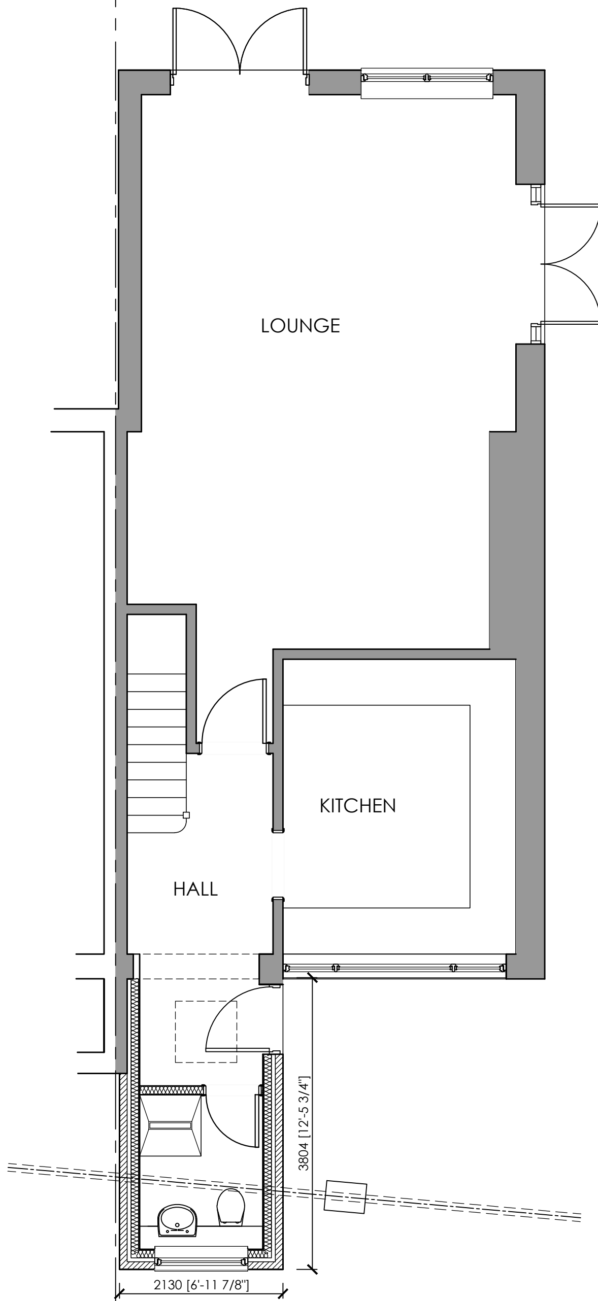
GROUND FLOOR PLAN AS PROPOSED 1:50
