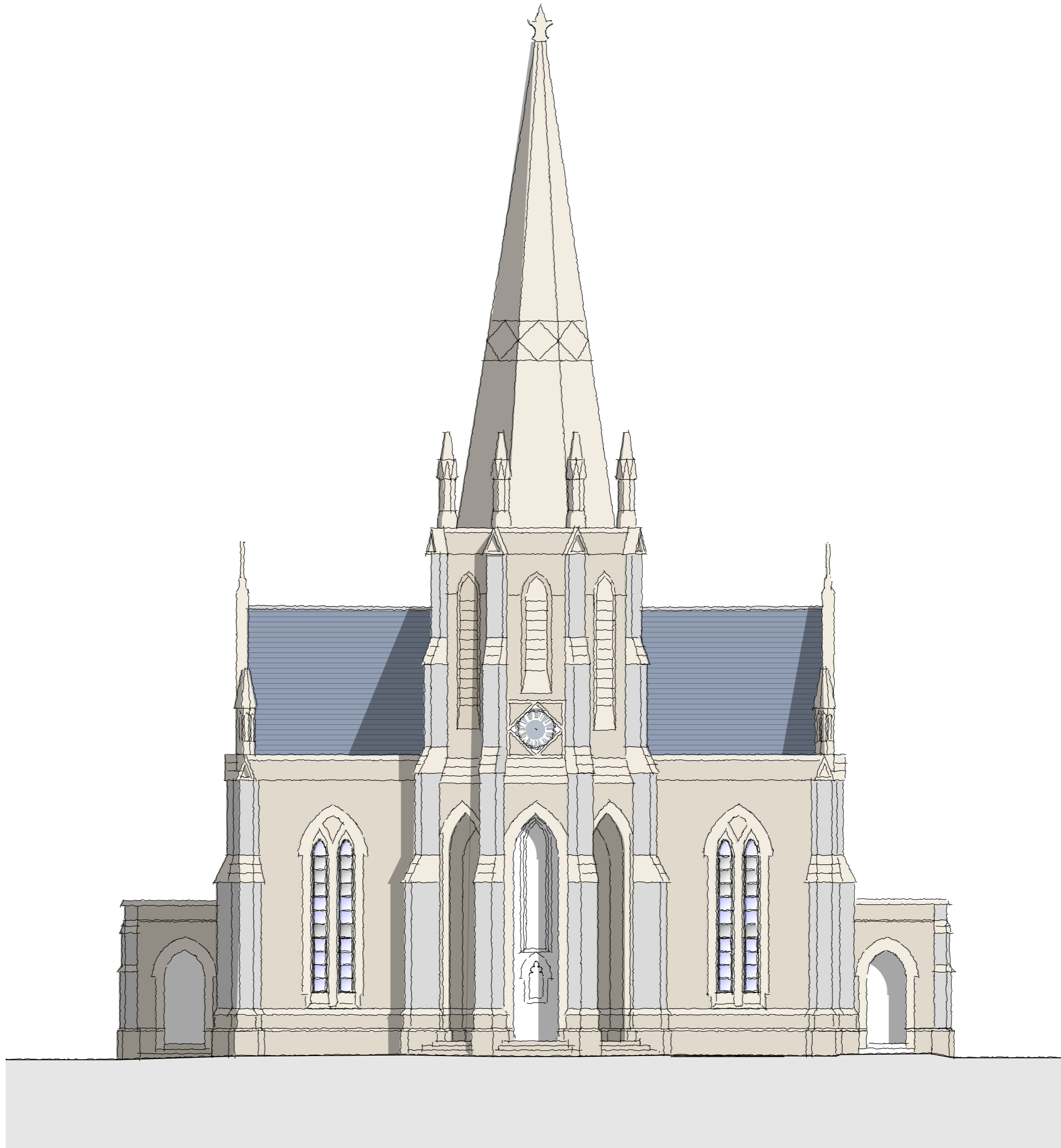
NORTH EAST ELEVATION
