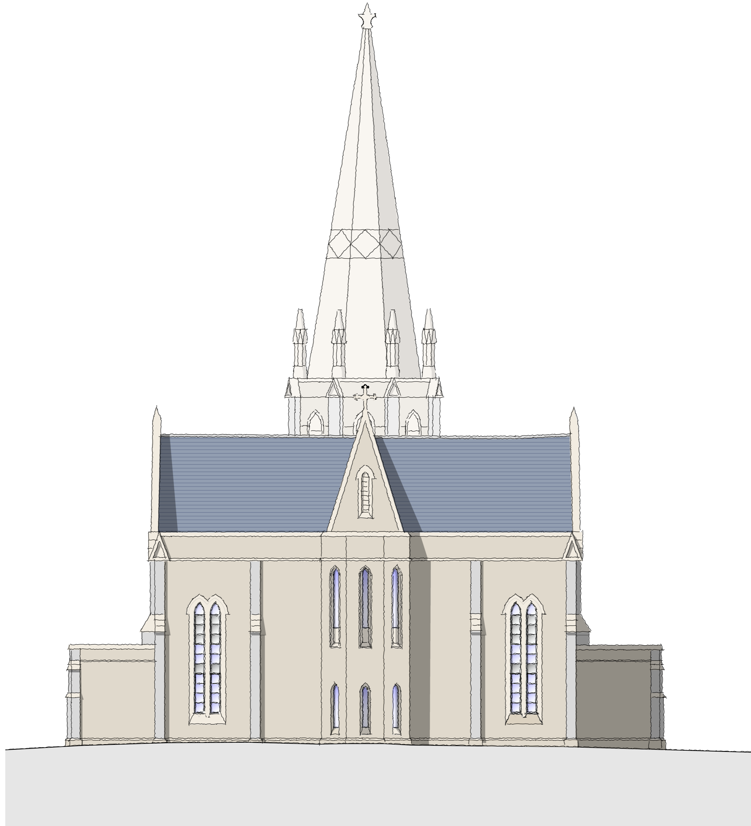
SOUTH WEST ELEVATION
