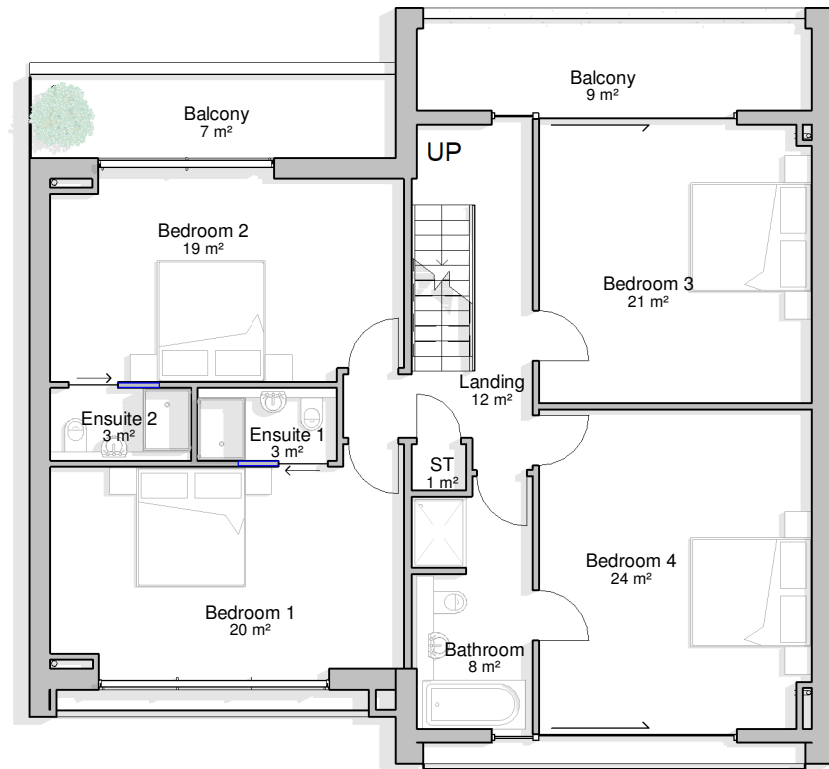
First Floor Site Plan 1 : 125
