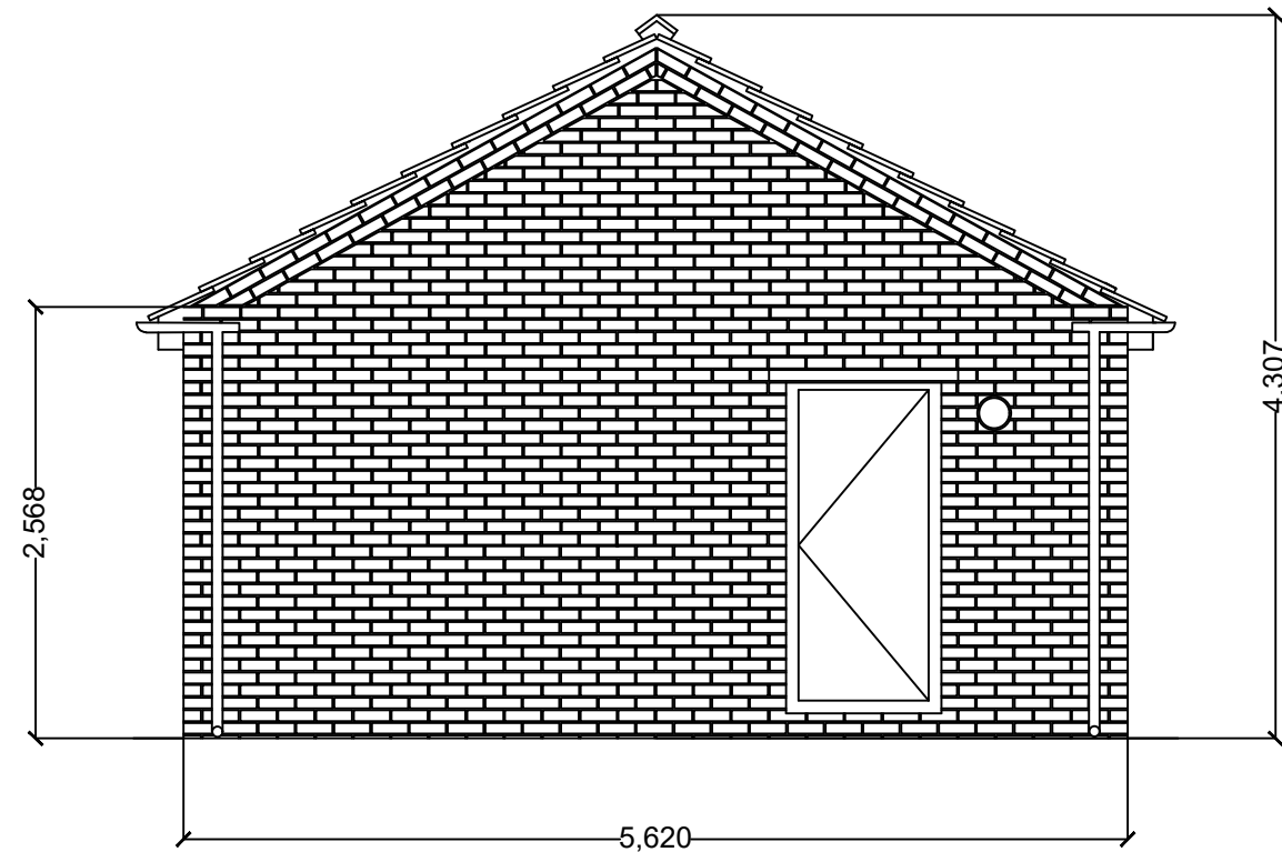
West Elevation
