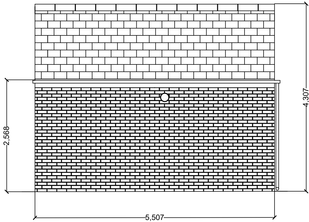
North Elevation
