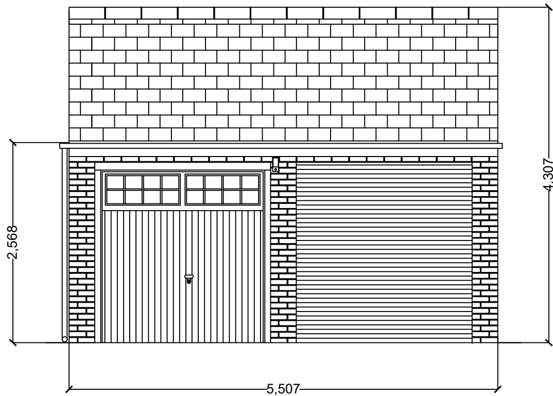
South Elevation
