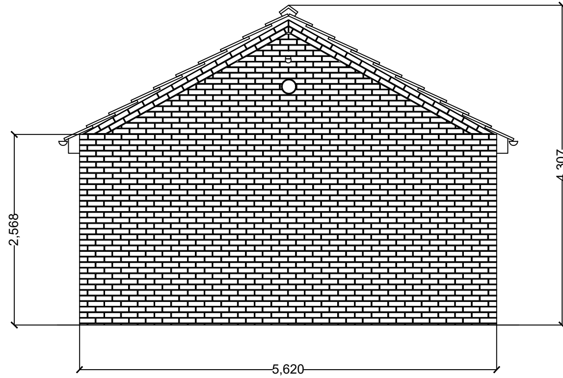
East Elevation
