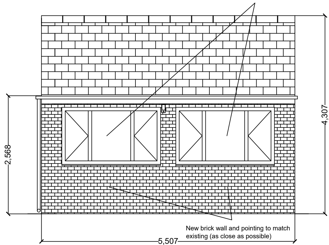
South Elevation
