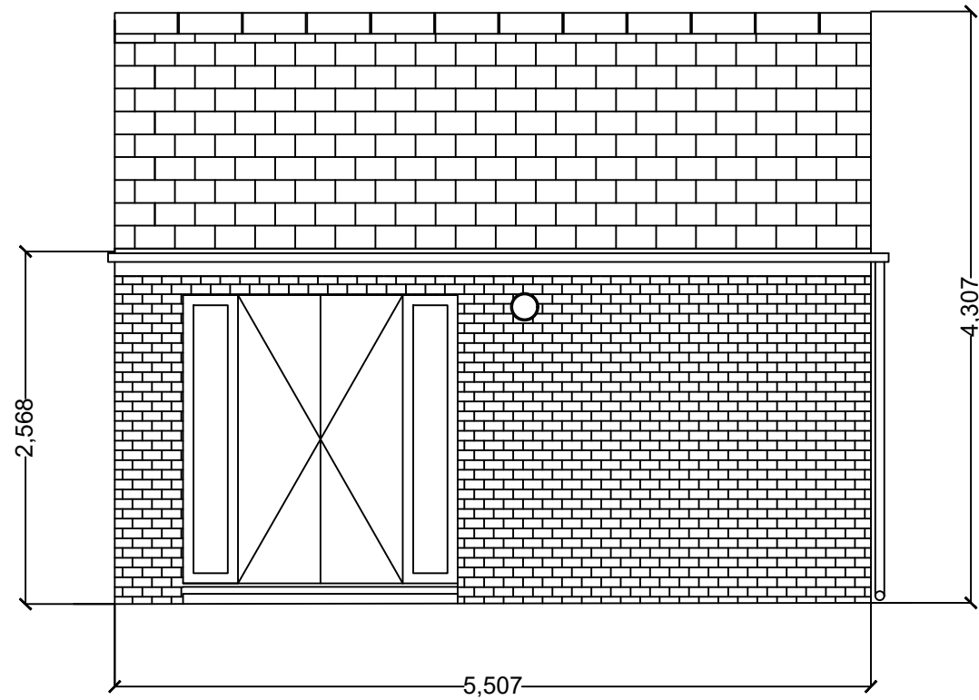
North Elevation
