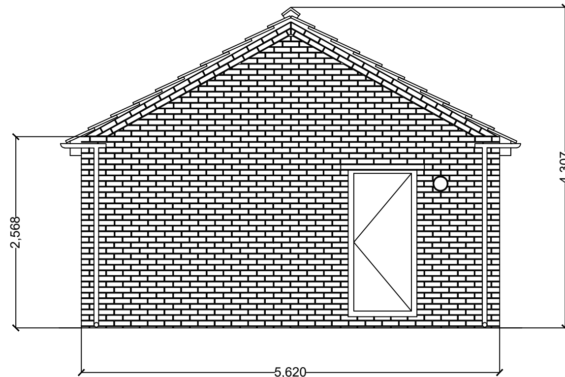
West Elevation
