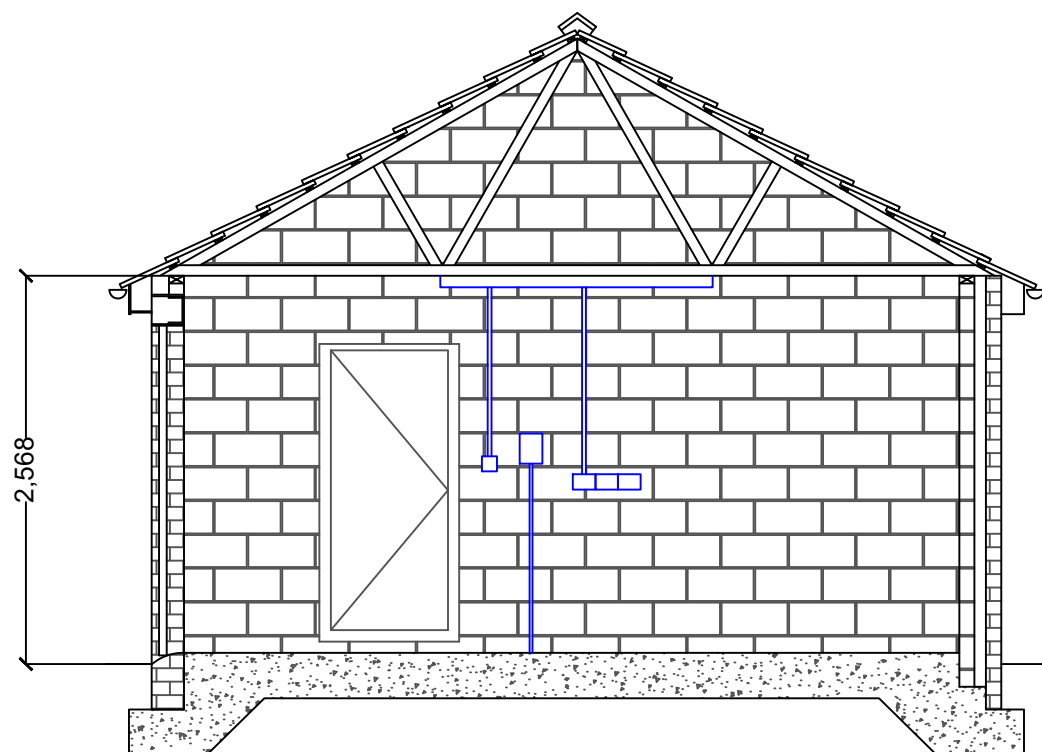
East Elevation - Section - Existing - A-A
