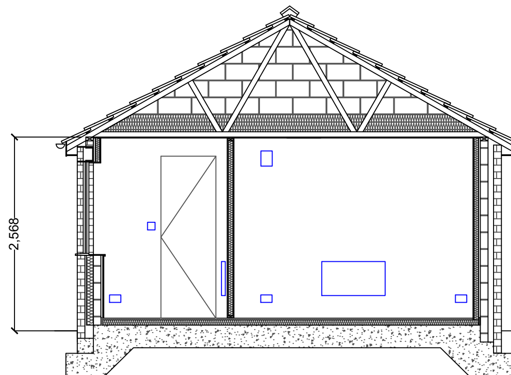
East Elevation - Section - Proposed - A-A
