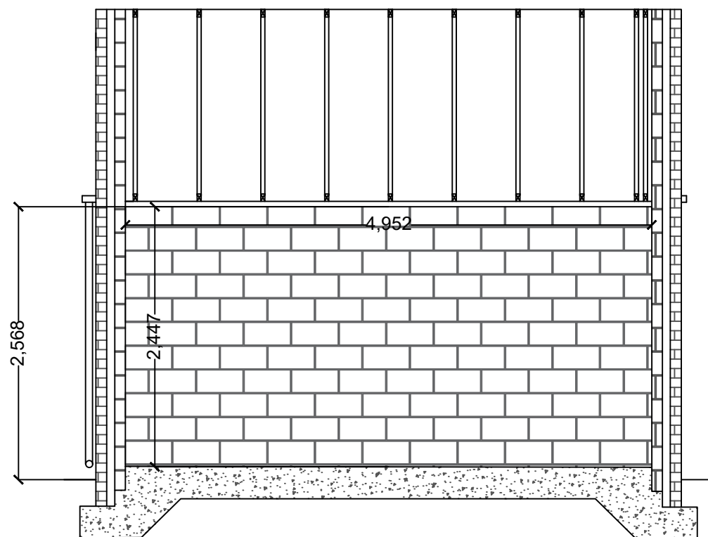
South Elevation - Section - Existing - B-B
