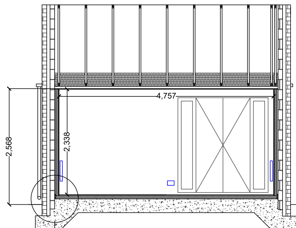
South Elevation - Section - Proposed - B-B
