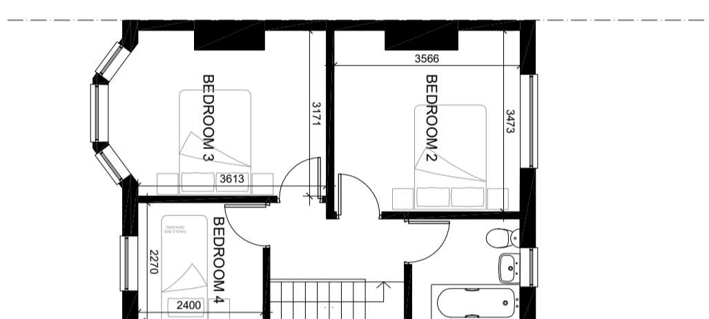
FIRST FLOOR PLAN AS EXISTING
