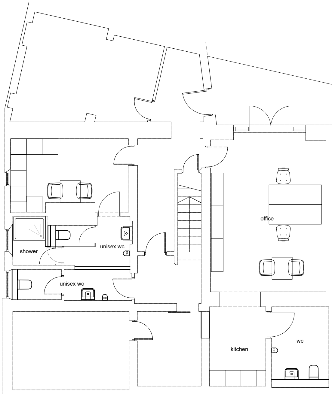
Proposed Basement Plan - 1:50
