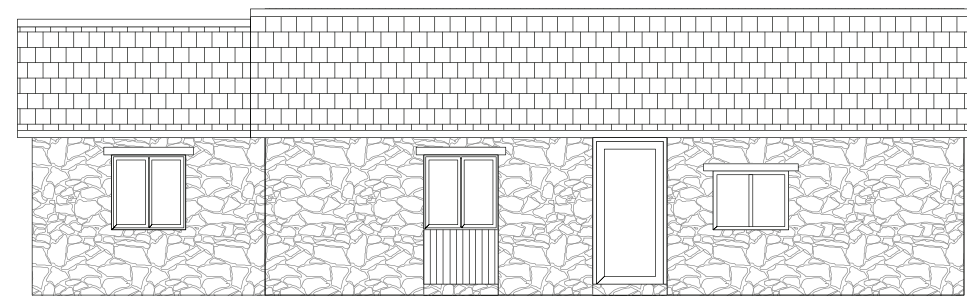
FRONT ELEVATION
