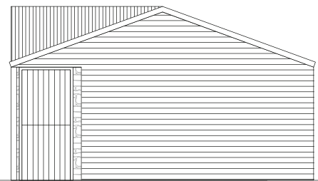
Side (South) Elevation
