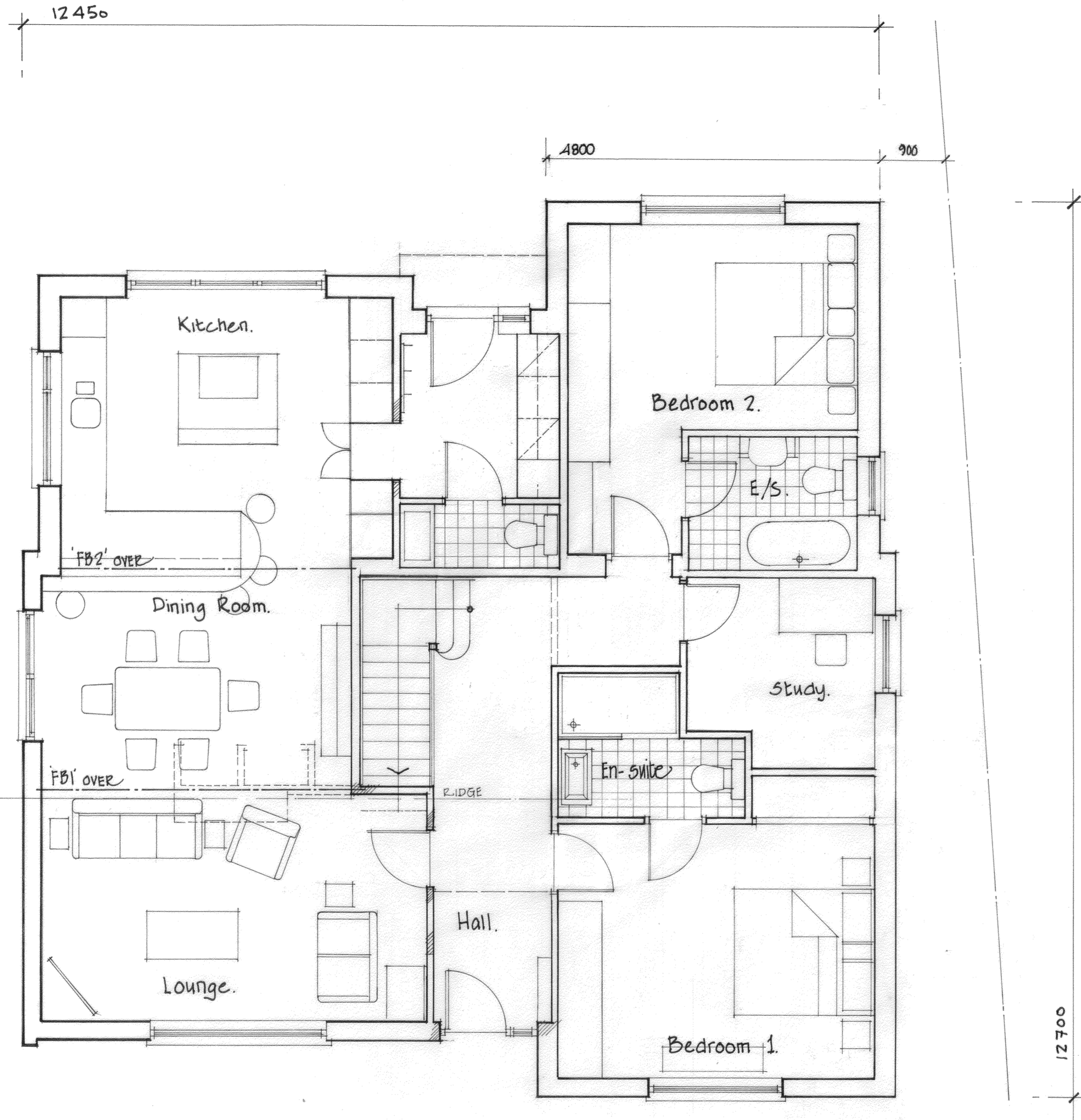
GROUND FLOOR AS PROPOSED
