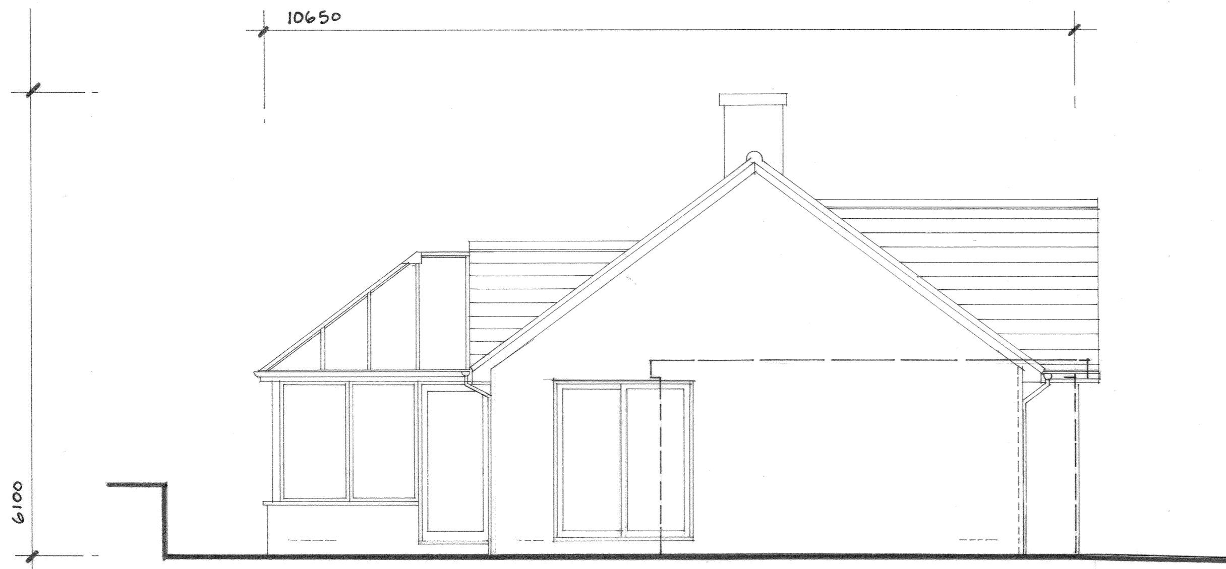
NORTH WEST ELEVATION AS EXISTING
