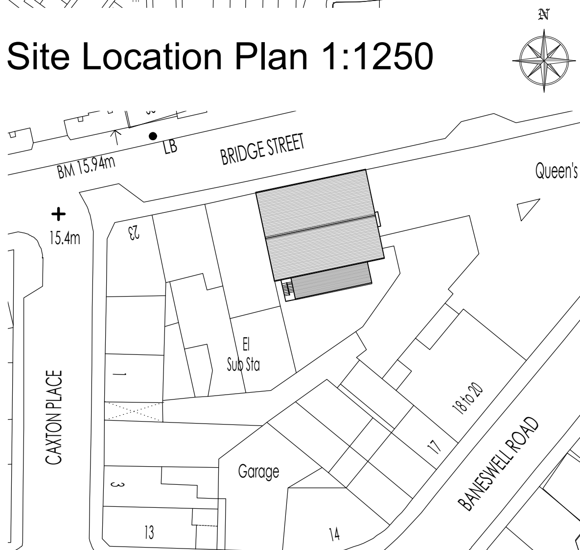
Existing Site Block Plan 1:500
