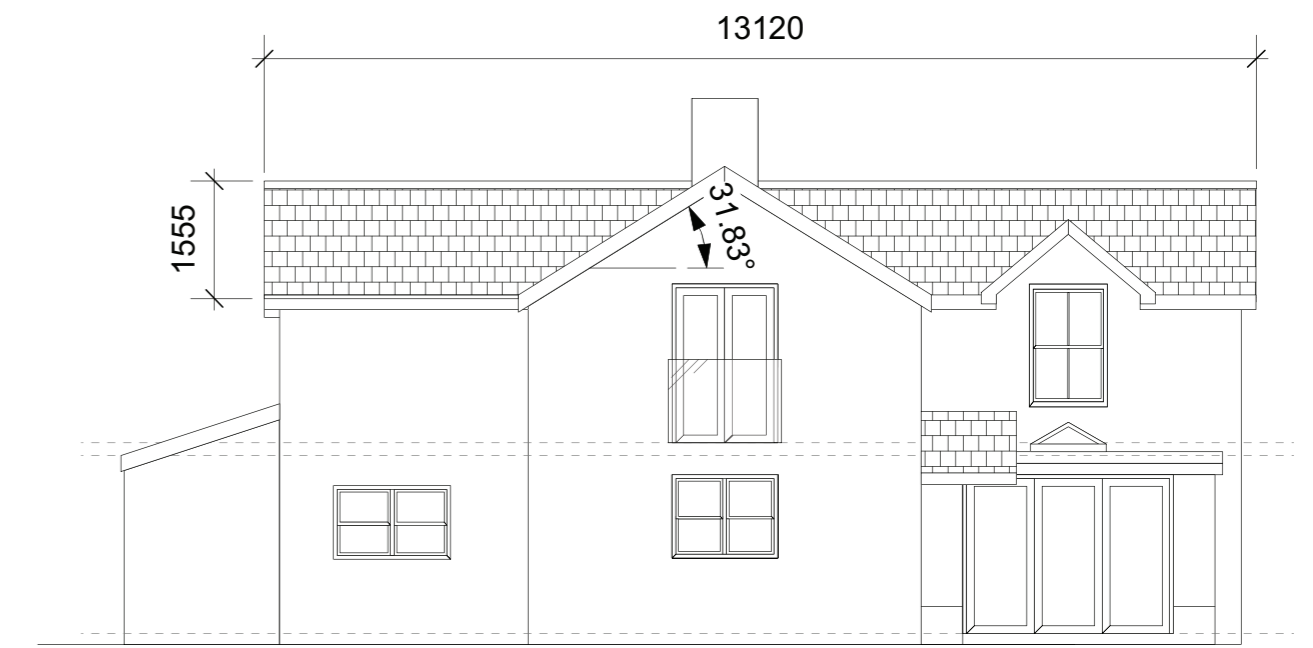
SIDE (WEST) ELEVATION
