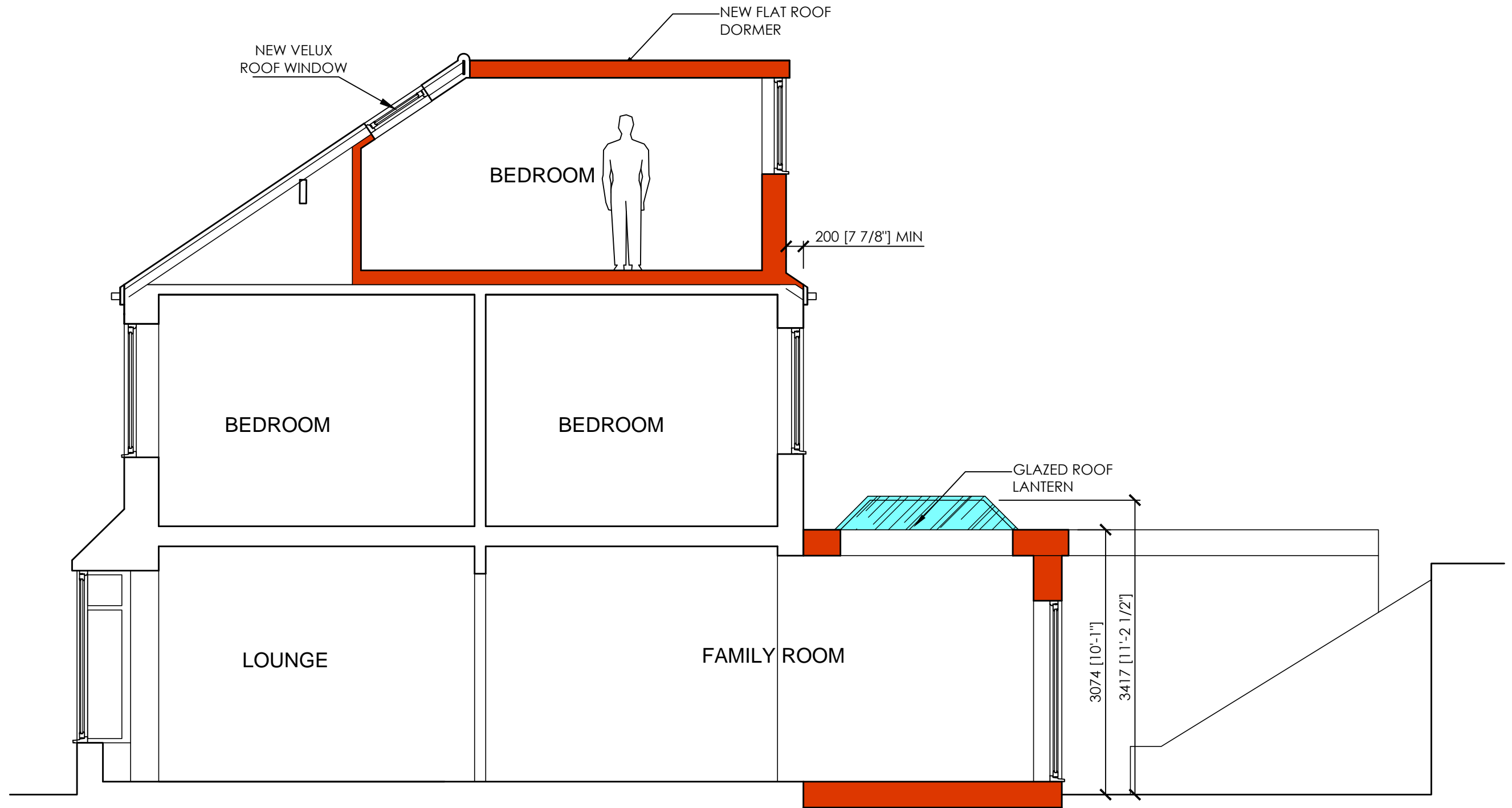
SECTION A-A AS PROPOSED
