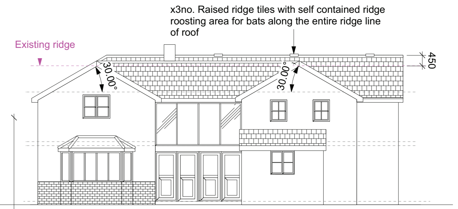
REAR ELEVATION
