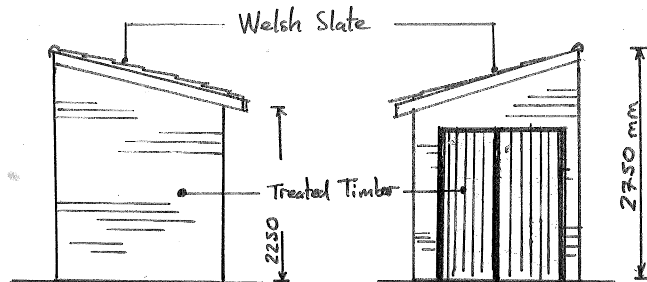
END ELEVATION ROAD SIDE
