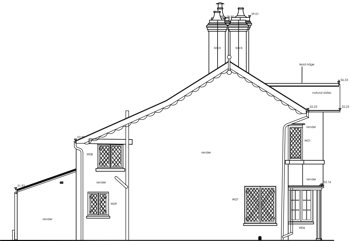
North Elevation
