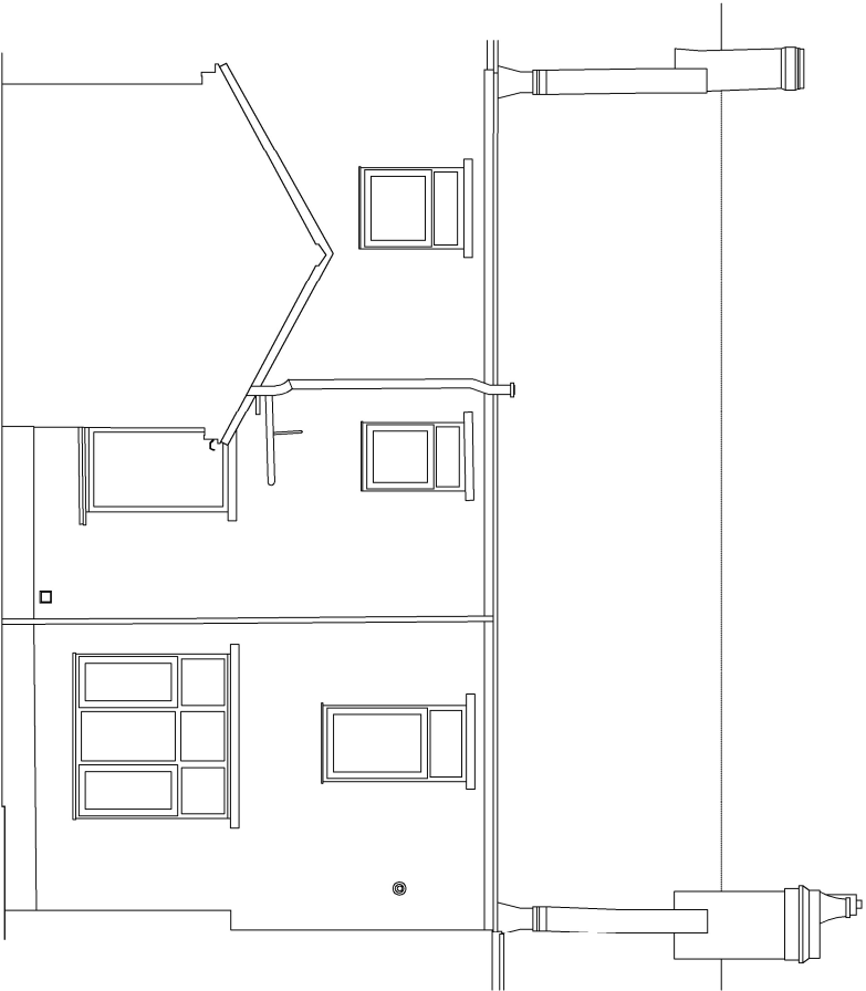
Existing Elevation B 1:100
