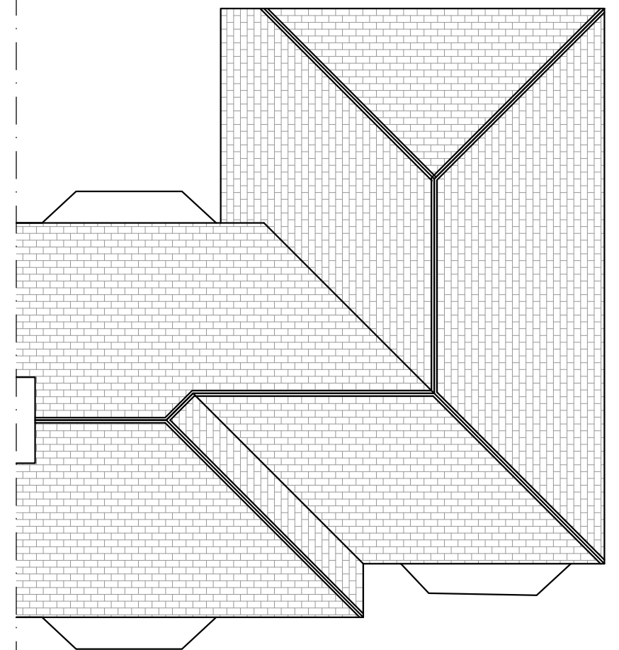
ROOF PLAN AS PROPOSED 1:100
