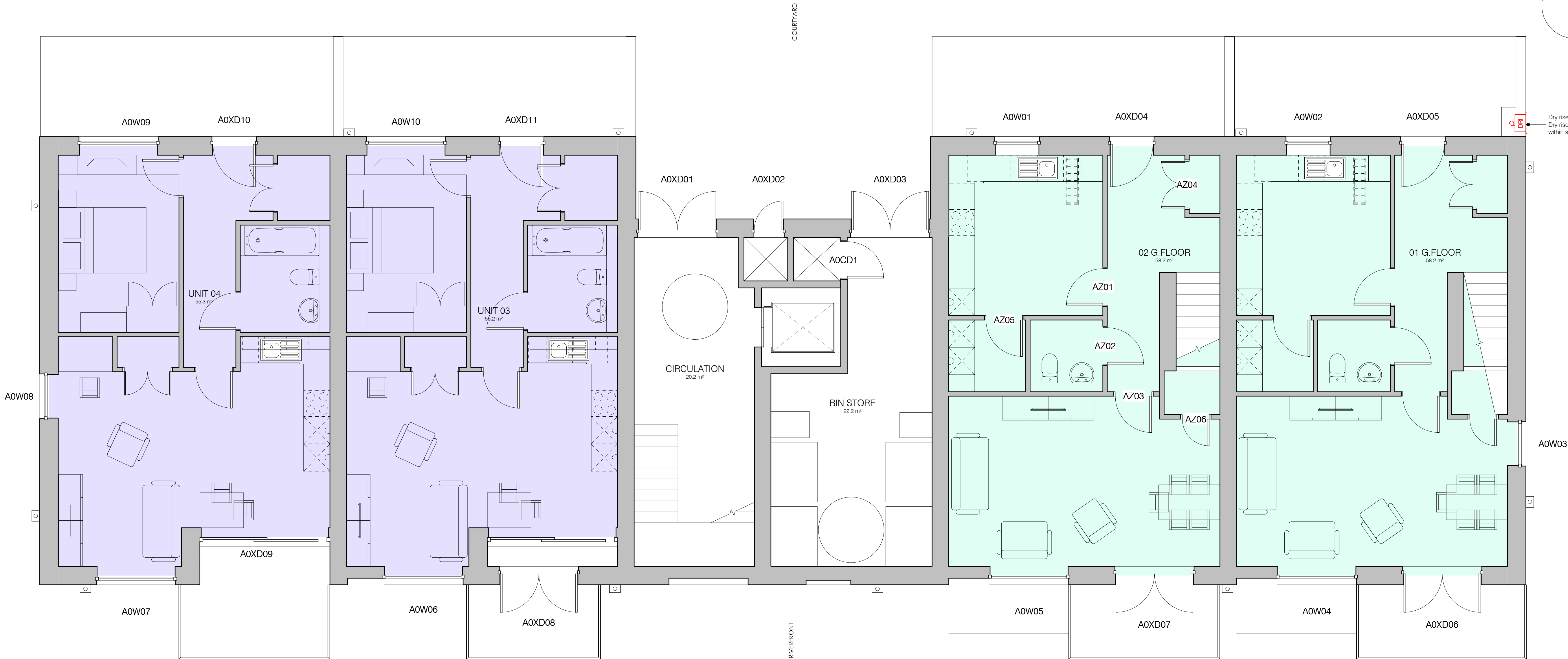
00 Ground Floor GA Plan 1 : 50
