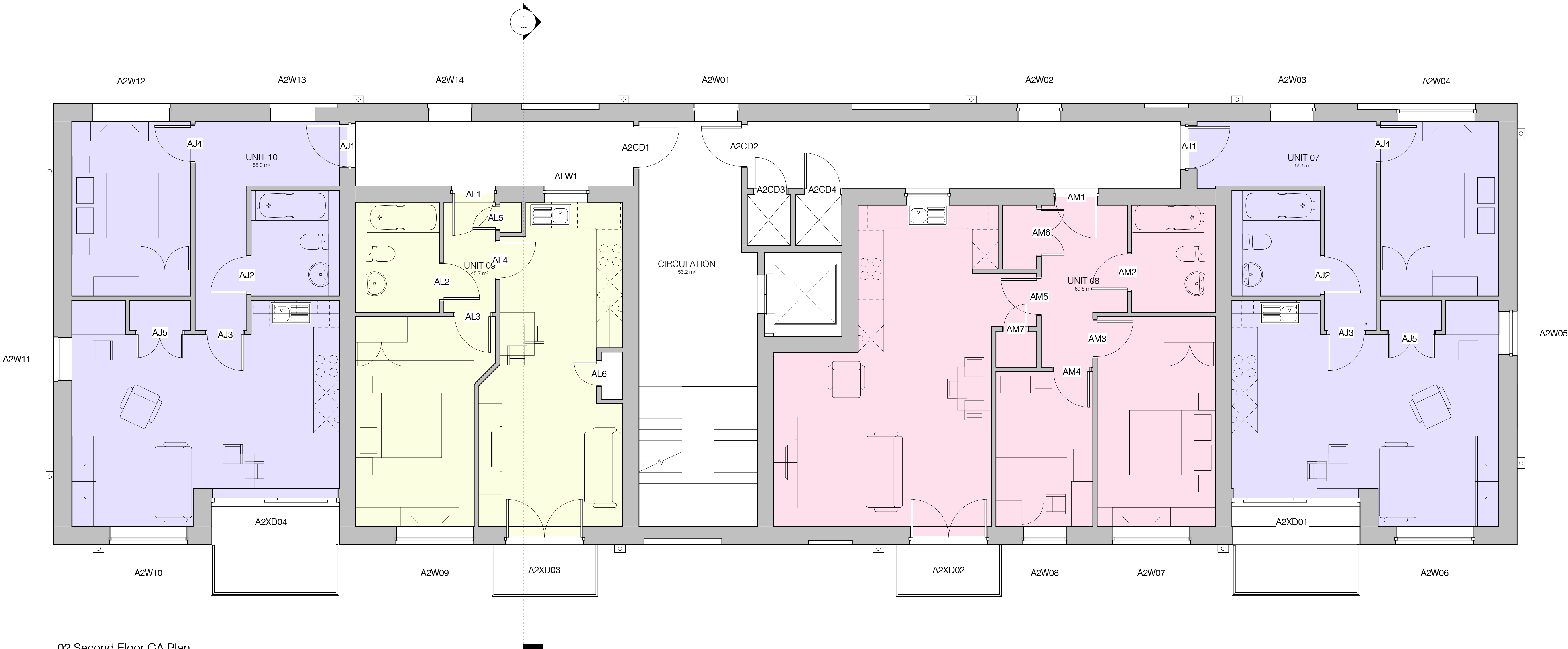
02 Second Floor GA Plan
