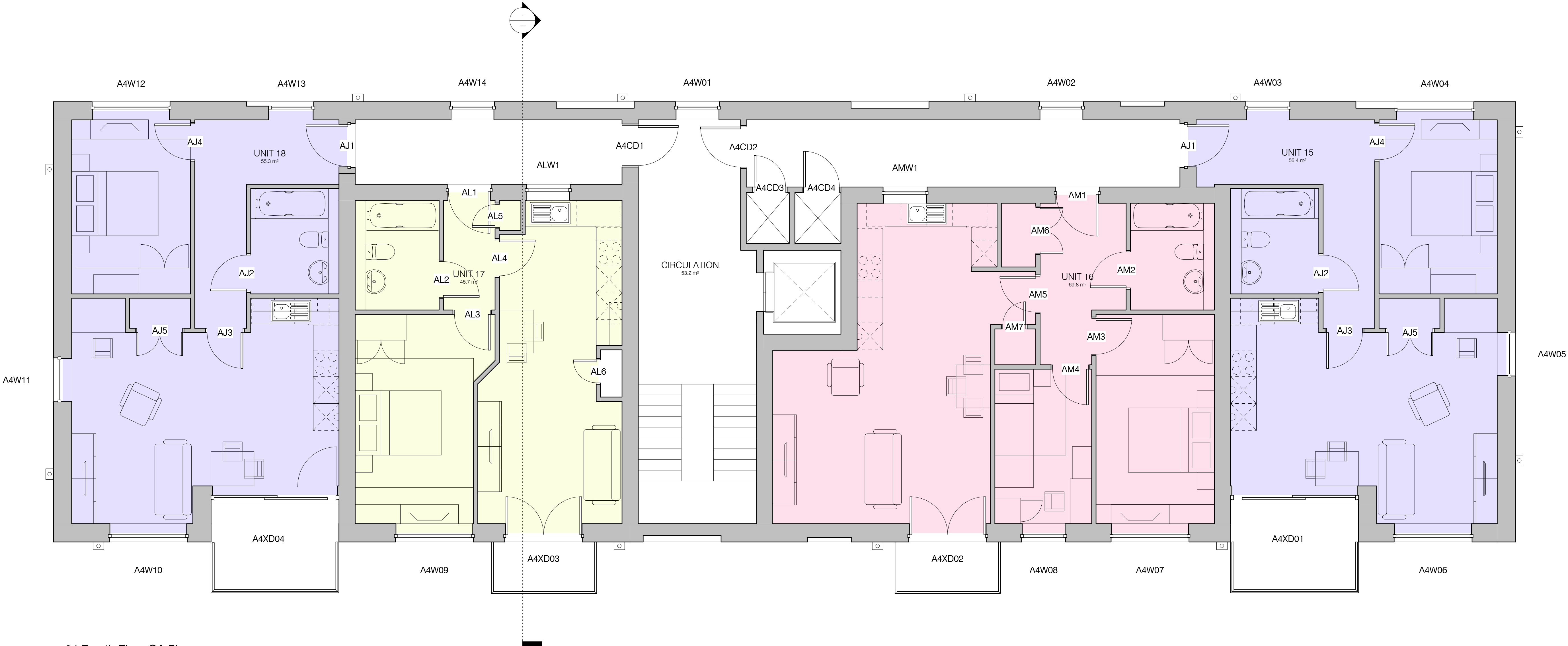
04 Fourth Floor GA Plan 1 : 50
