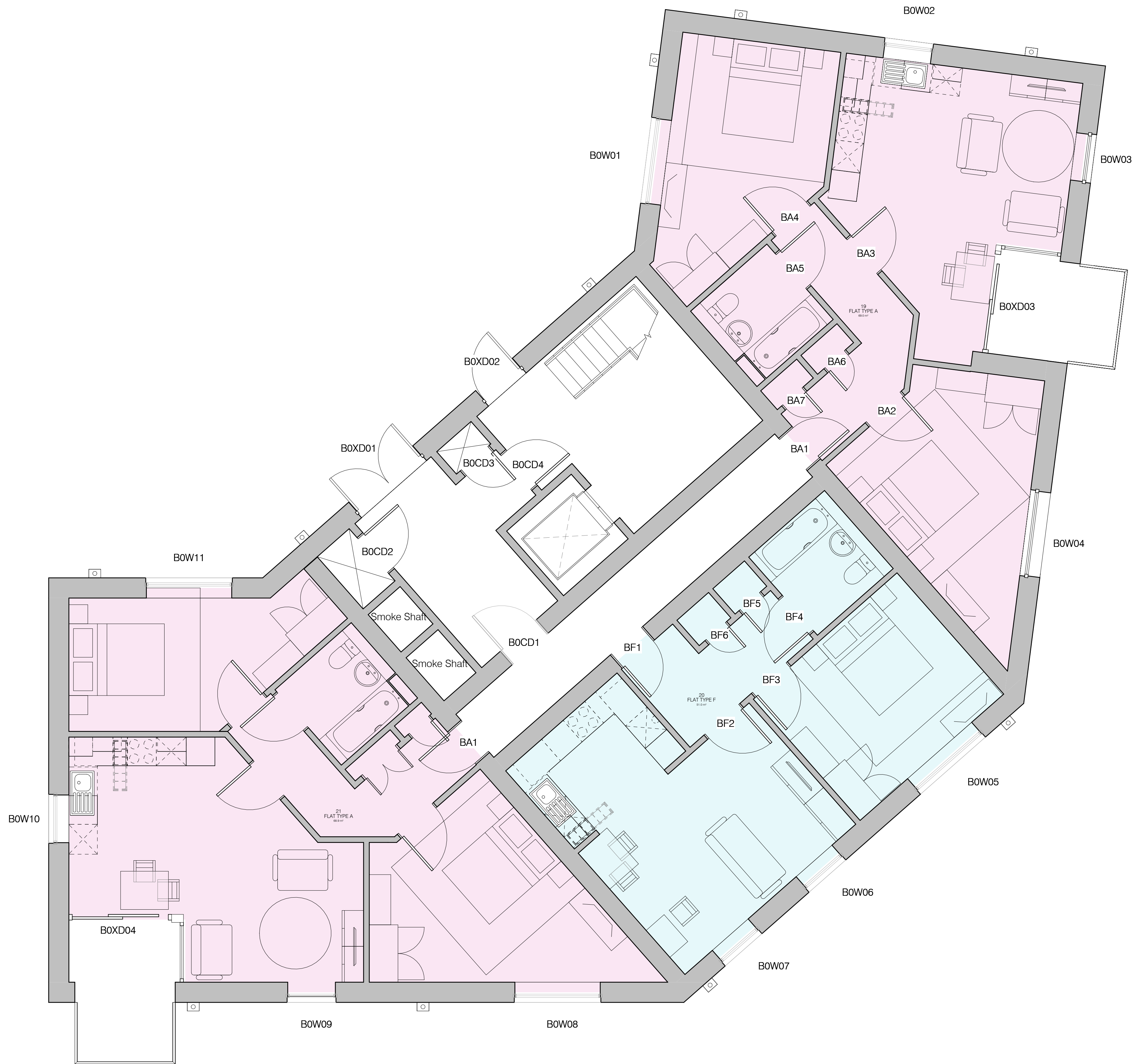
00 Ground Floor GA Plan 1 : 50
