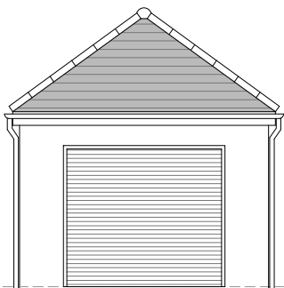
PROPOSED FRONT ELEVATION
