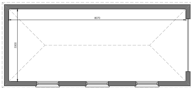
PROPOSED GARAGE PLAN
