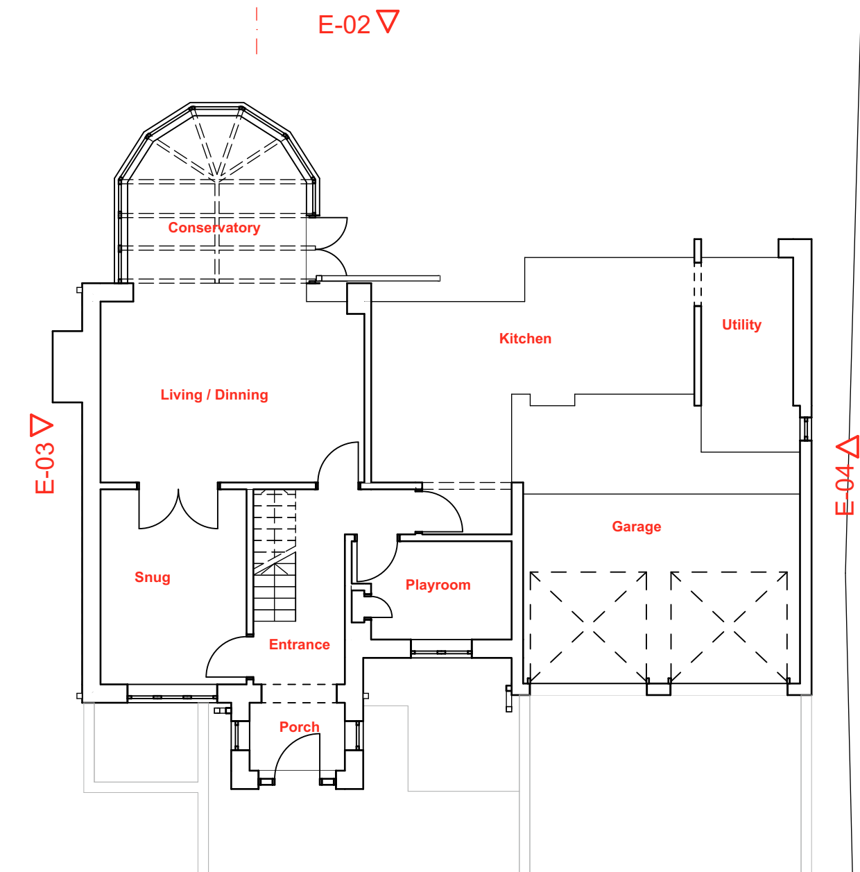
0. GF-Ground Floor 1:100
