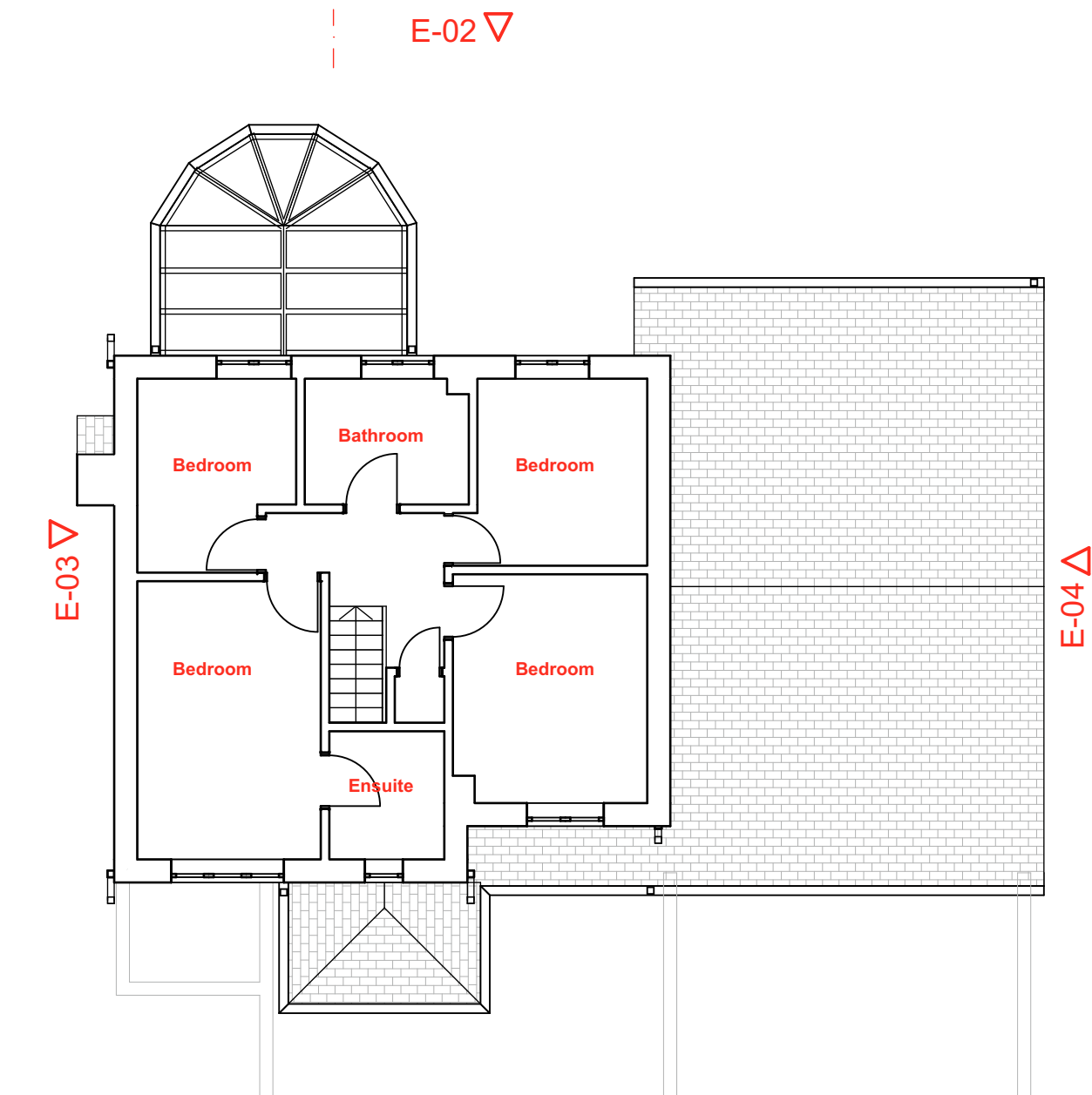
1. 01-First Floor 1:100
