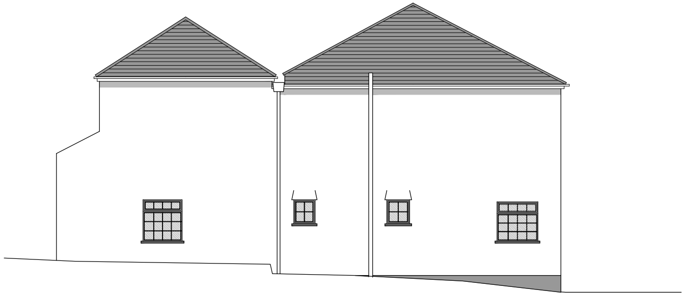
PROPOSED SIDE ELEVATION 1:100 @ A3
