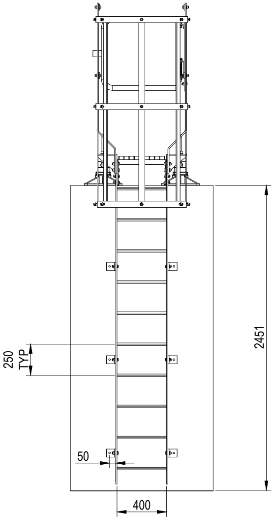
FRONT ELEVATION (1:30)
