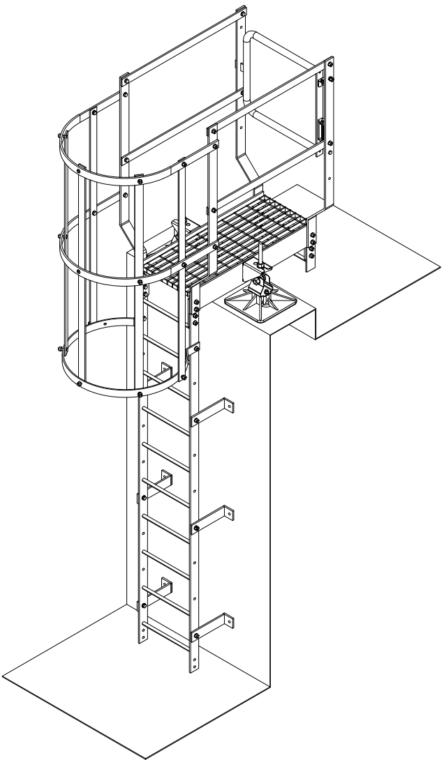
ISOMETRIC (1:30)
