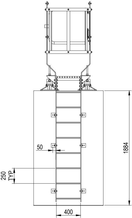
FRONT ELEVATION (1:30)
