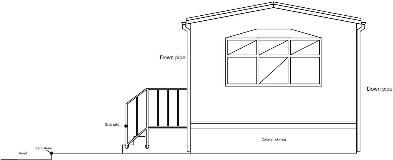
Side Elevation (B) - Existing
