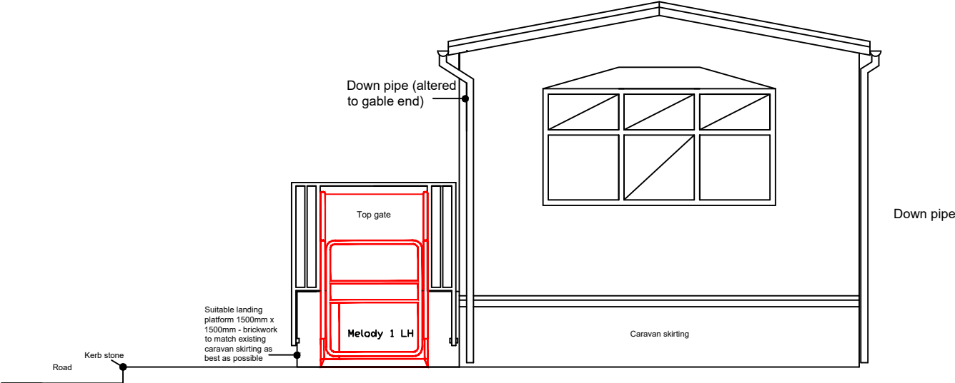
Side Elevation (B) - Proposed
