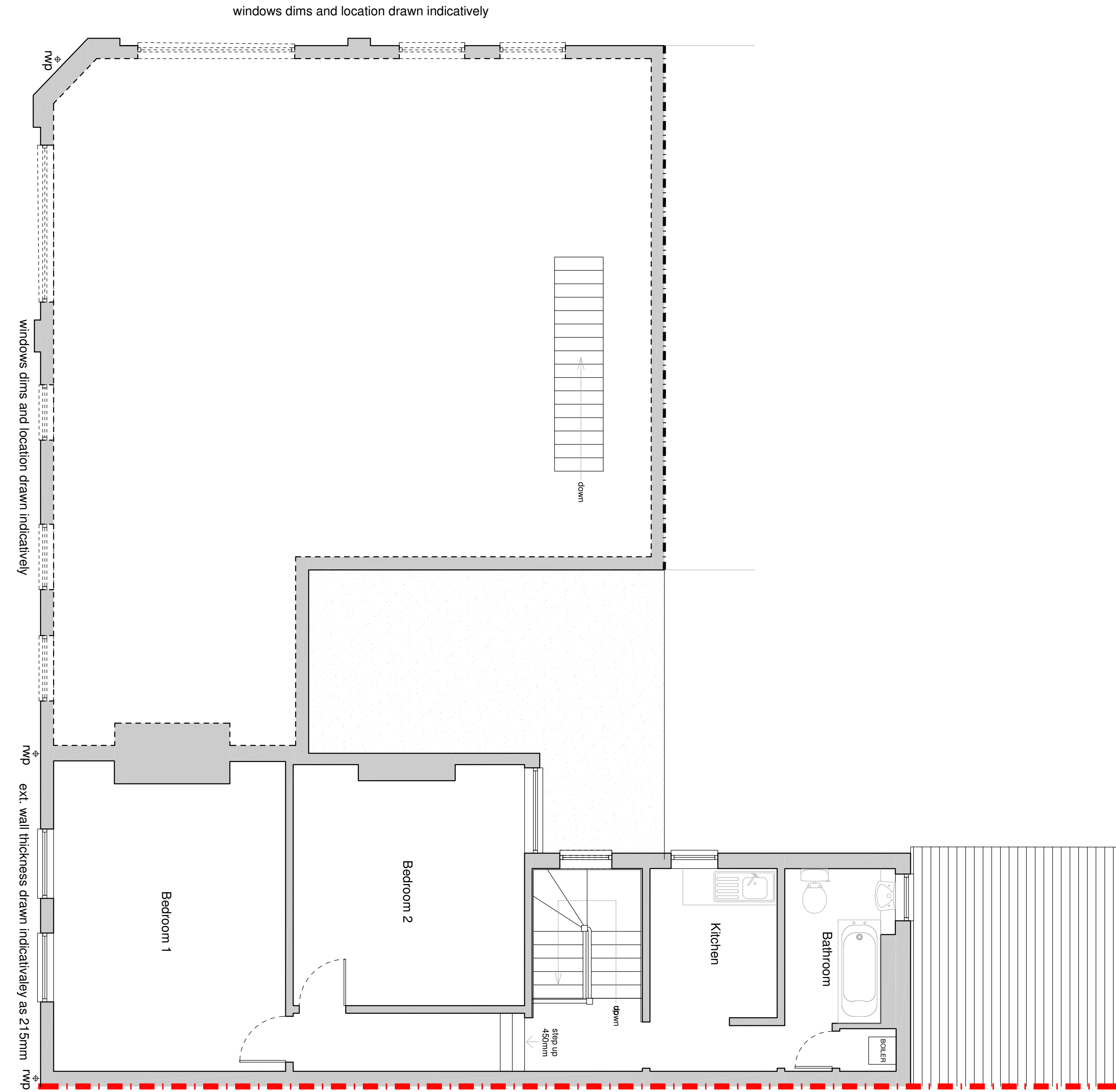
FIRST FLOOR
