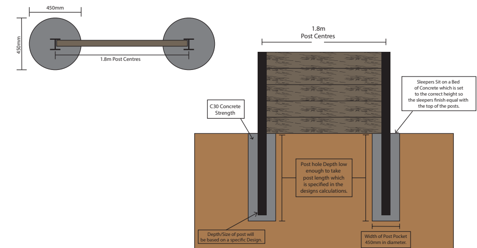
Cross Section Drawings
