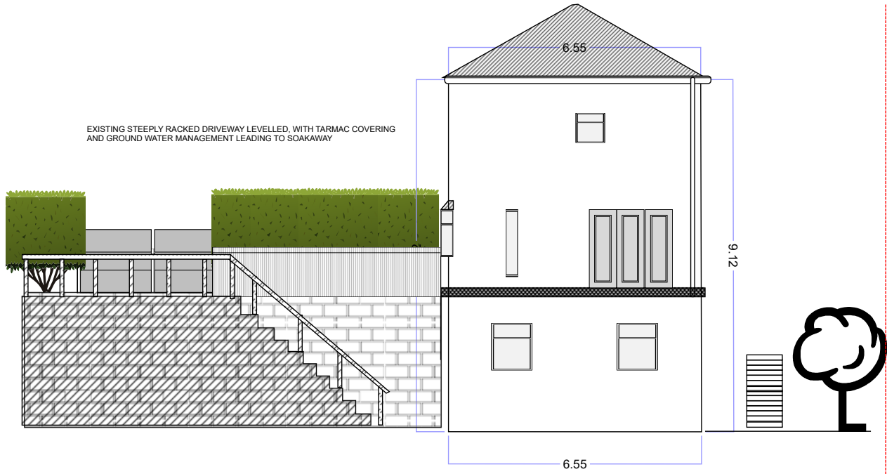
REAR (NORTH EAST) ELEVATION PROPOSED
