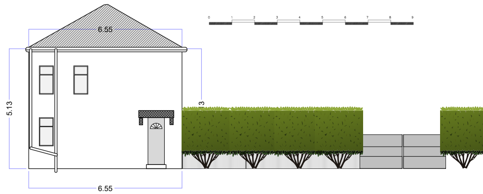
FRONT (SOUTH WEST) ELEVATION PROPOSED
