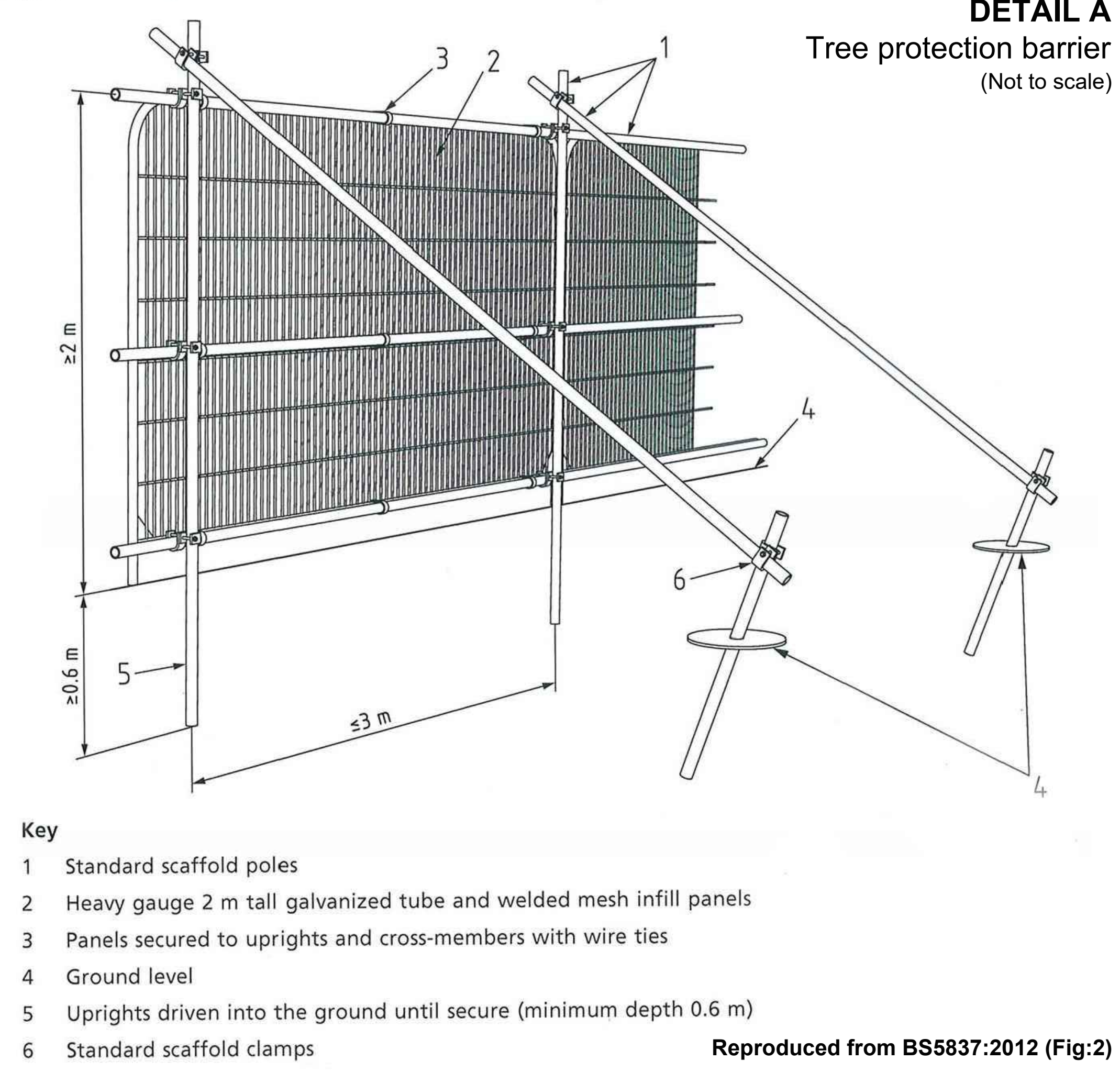
Figure 2 Default specification for protective barrier
