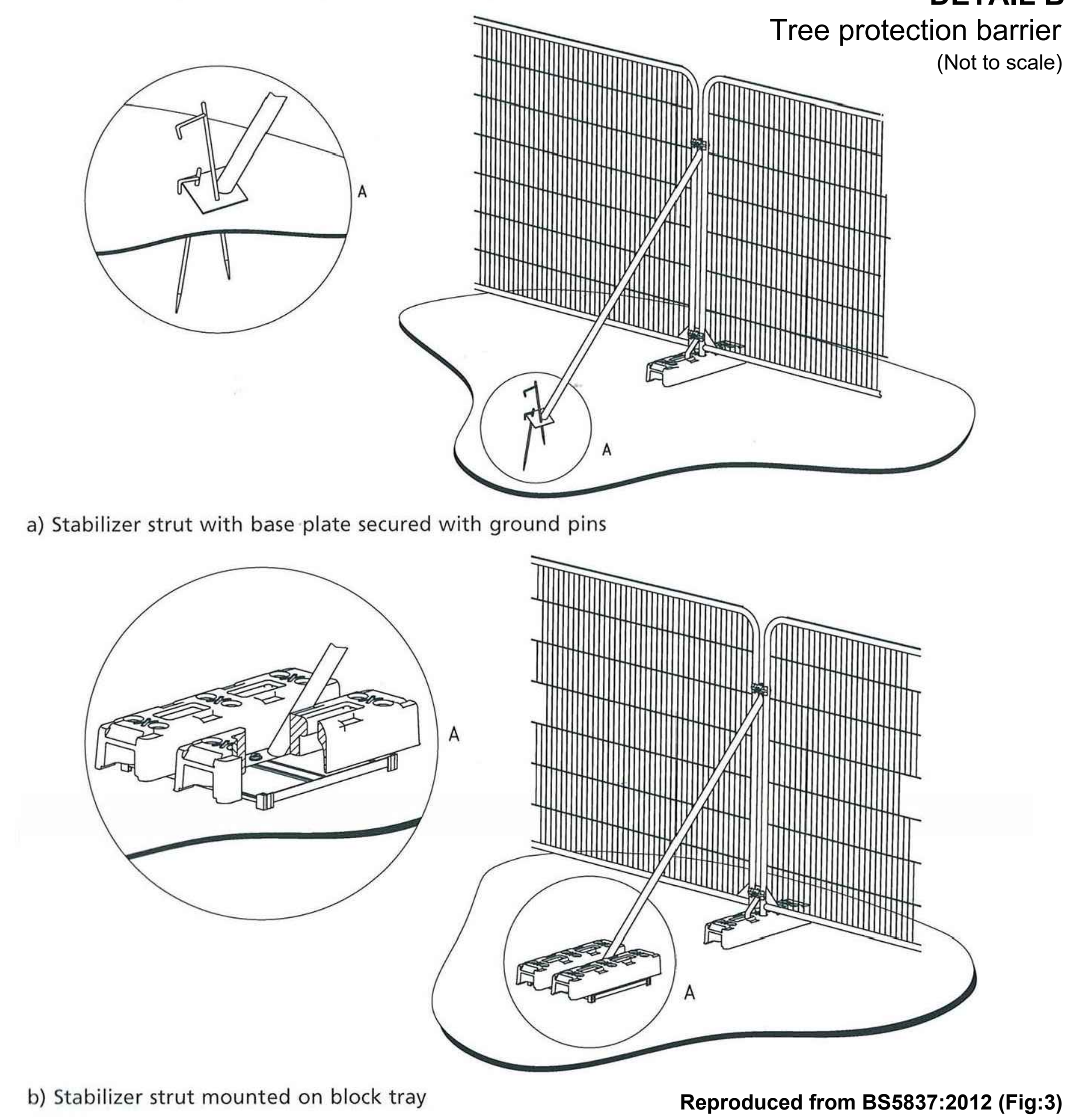
Figure 3 Examples of above-ground stabilizing systems
