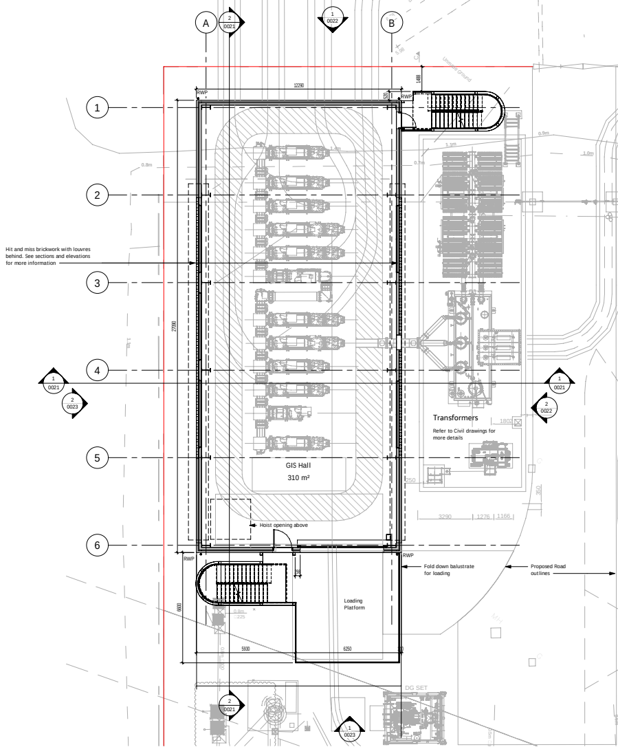
1 First Floor Level 1 : 100
