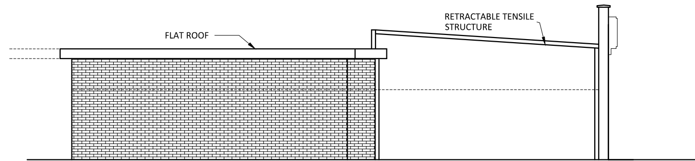
PROPOSED SIDE ELEVATION AA (RK PIZZA POINT SIDE)
