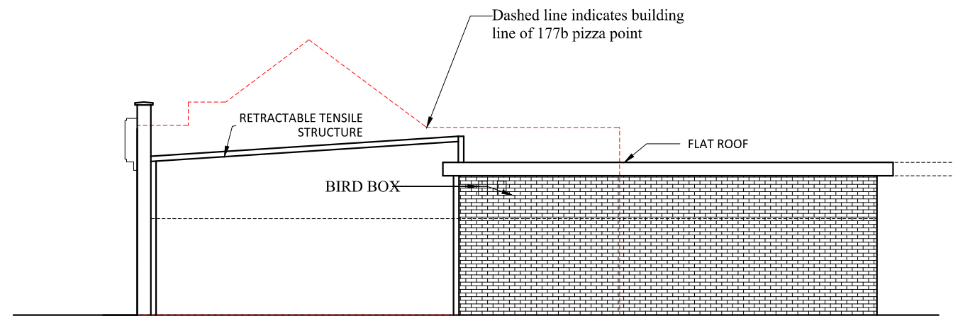
PROPOSED SIDE ELEVATION BB (THE VICTORIA INN SIDE)
