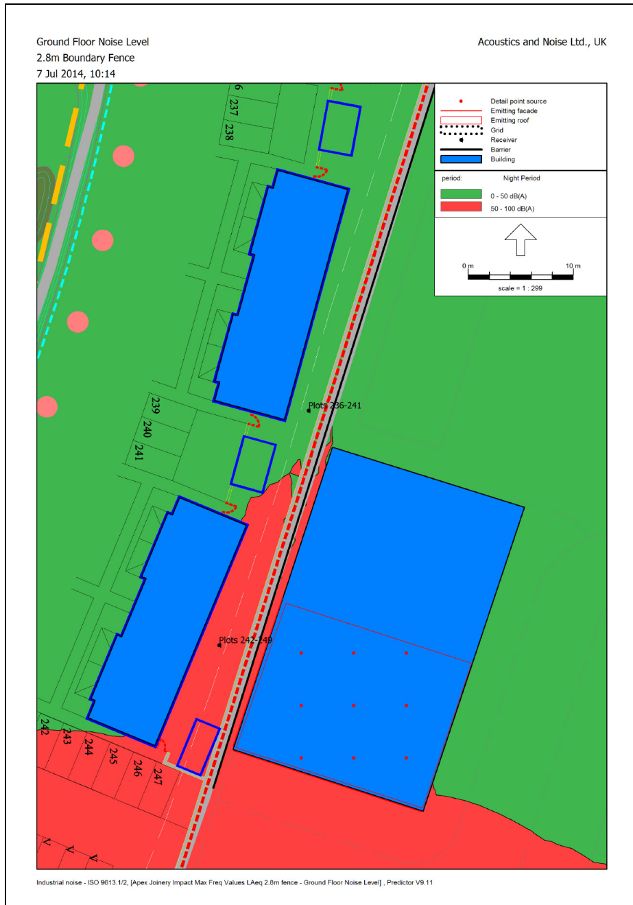
Figure 3 – Calculated External Noise Contours @1.5m
