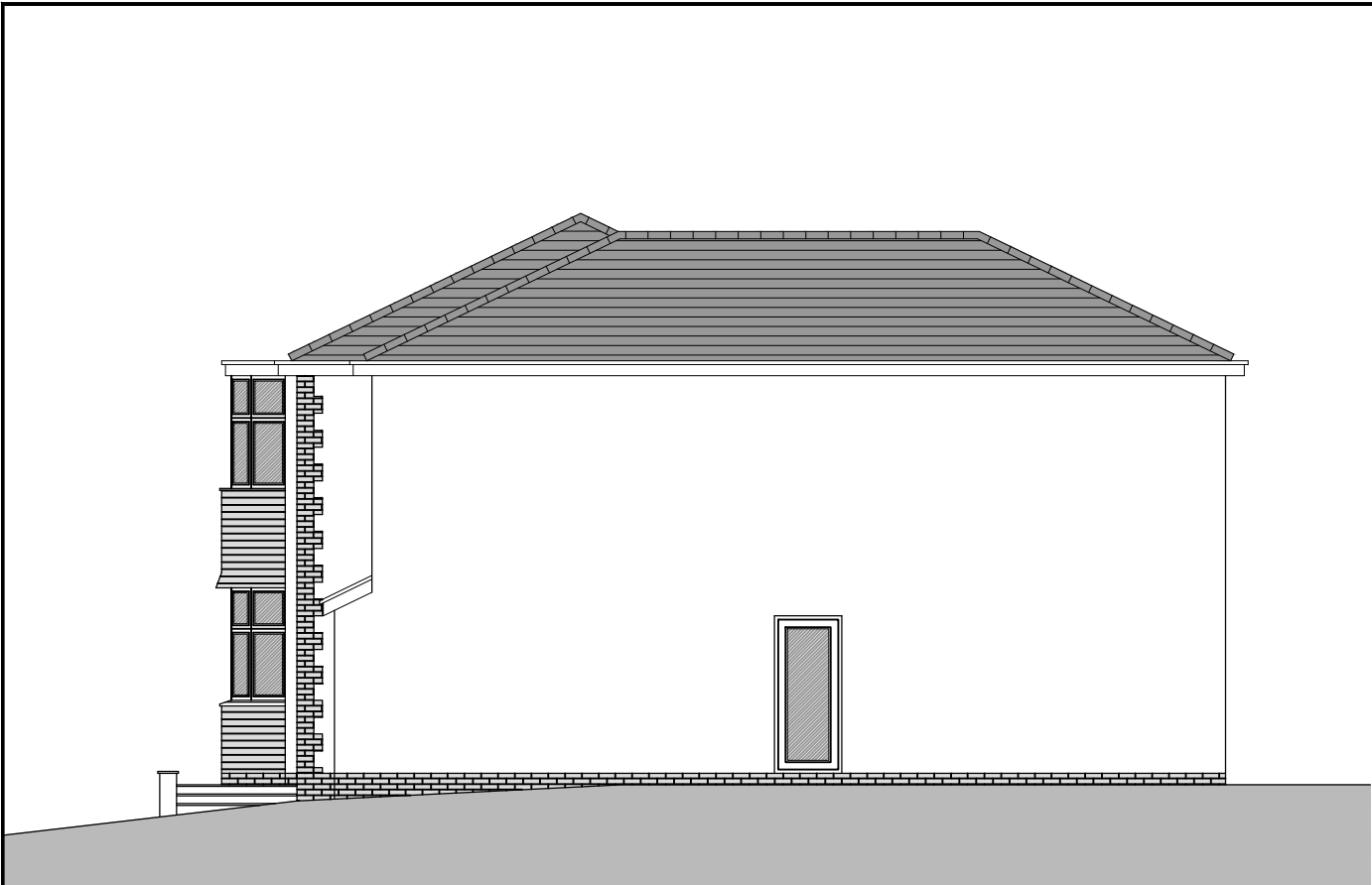
PROPOSED SIDE ELEVATION 1:100 @ A3
