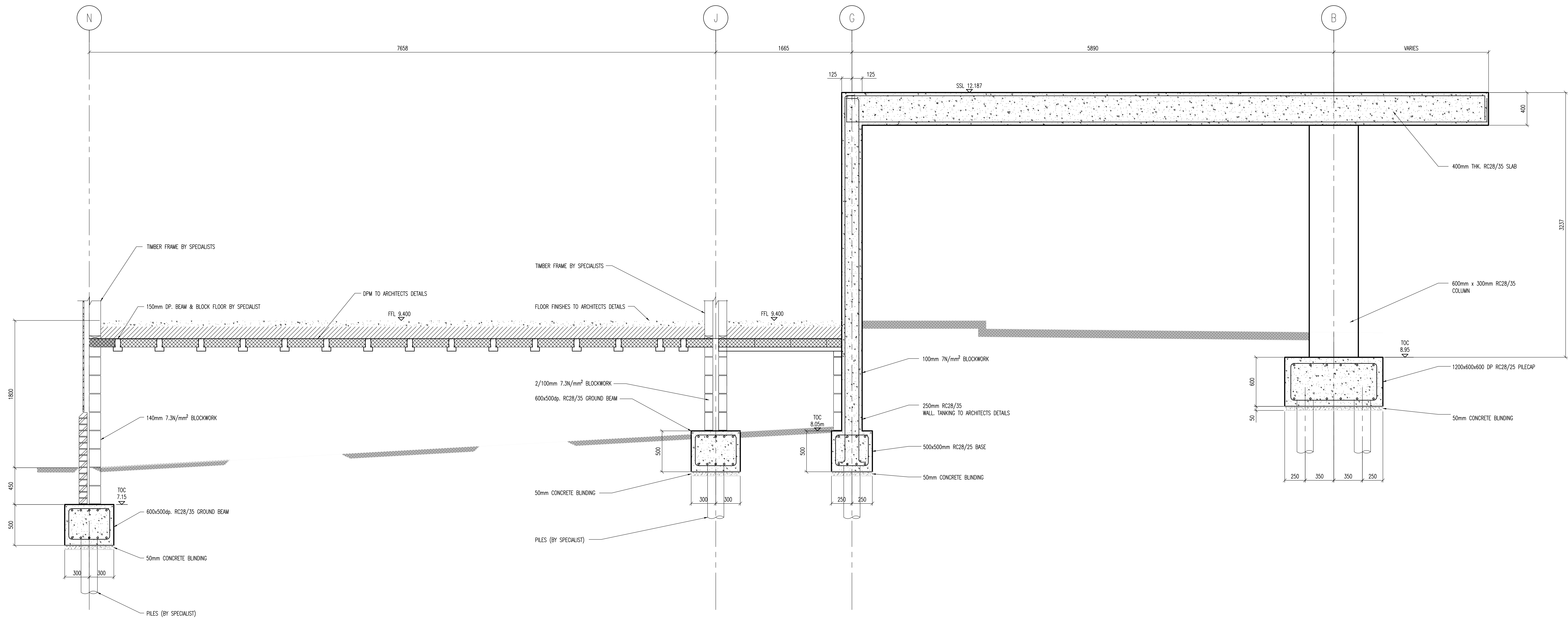
SECTION 1-1 SCALE 1:50
