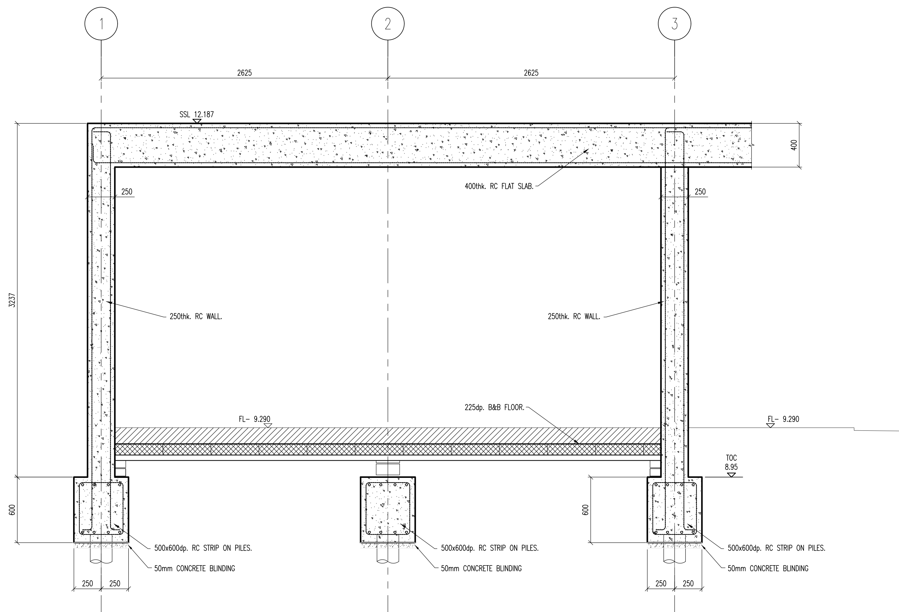
SECTION 2-2 SCALE 1:20
